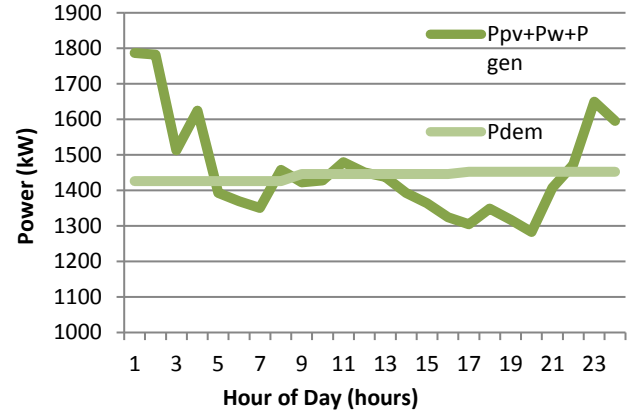
Figure 1: Generation and load profile for tanker operation during cargo unloading at port
