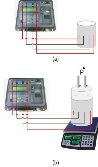
Fig. 4. PVC cell connected to electrical resistivity meter: (a) R_m \times w \times \delta and (b) R_m \times C \times \delta .
