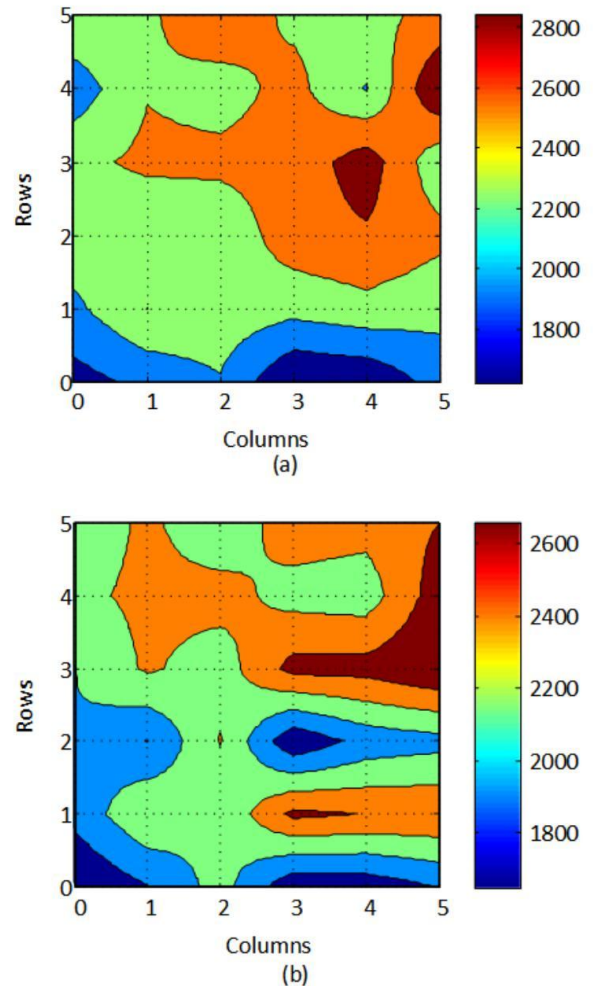
Fig. 10. Moisture stains mapping through Lateral Profiling method ( \rho_a ).
