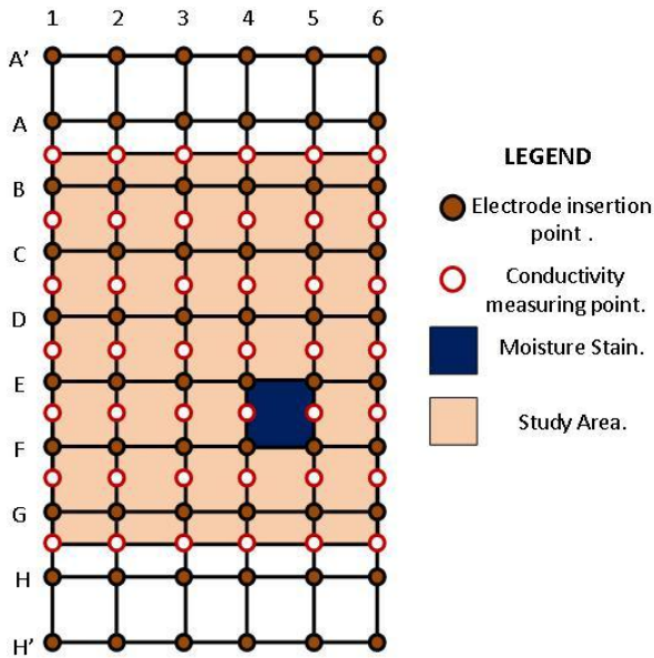
Fig. 5. Delimited area for the application of Lateral Profiling method.
