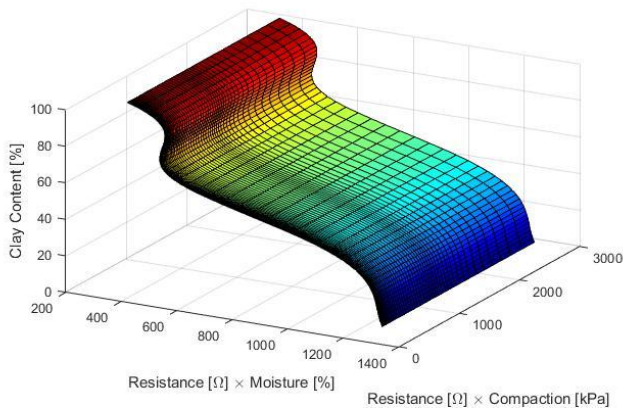
Fig. 9. Correlation Surface.
